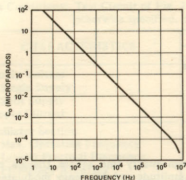
Figure 4. Frequency as a Function of C_O Across Pins 14 and 15
